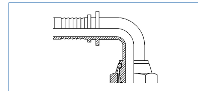
Female Swivel 24° 90° Elbow & O-Ring
