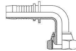
BSPP Swivel Female 90° Elbow
