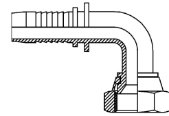
Female JIC 90°
