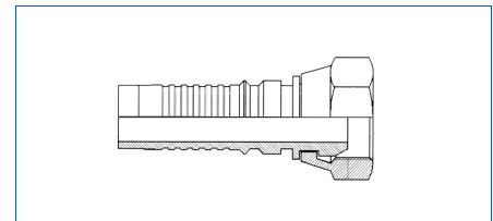
Female BSPP Interlock
