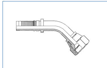
Female JIC 45° Interlock
