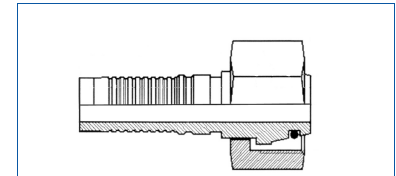
Female DIN2353 Interlock
