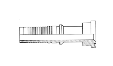
Code 61 Flange Interlock
