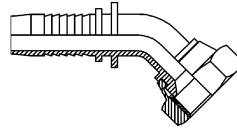
Female JIC 45°
