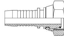
Female Swivel 24° with O-Ring
