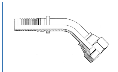
Female JIC 45° Interlock
