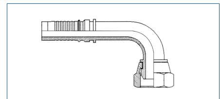
Female BSPP 90° Interlock
