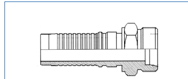
Male DIN2353 S Series Interlock
