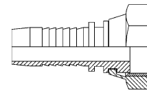
BSPP Swivel Female Flat Seat
