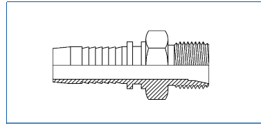
Metric Male 24°
