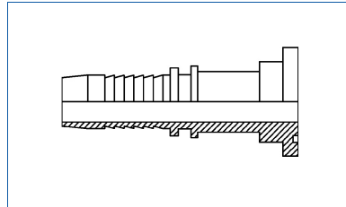
Code 62 Flange
