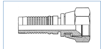
Female JIC Interlock
