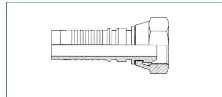
Female BSPP Interlock
