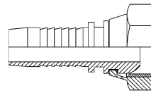
BSPP Swivel Female
