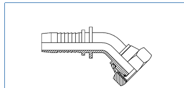
Female Swivel 24° 45° Elbow & O-Ring
