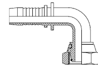
Female Swivel 24° 90° Elbow & O-Ring
