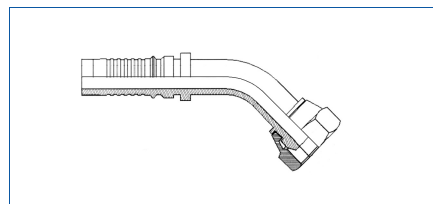
Female BSPP 45° Interlock
