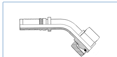
Female DIN2353 45° Interlock
