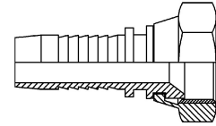
Female JIC
