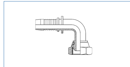
BSPP Swivel Female 90° Elbow
