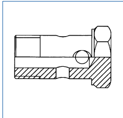
Banjo Bolt
