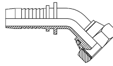
BSPP Swivel Female 45° Elbow
