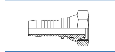
Female Swivel 24° with O-Ring
