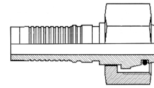
Female DIN2353 Interlock
