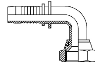
Female JIC 90°
