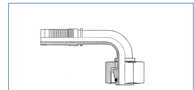
Female DIN2353 90° Interlock
