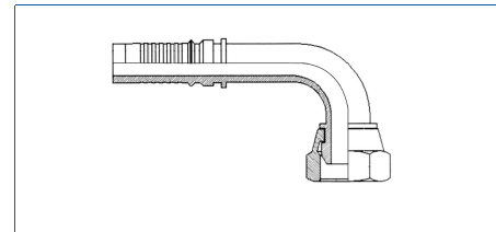
Female BSPP 90° Interlock
