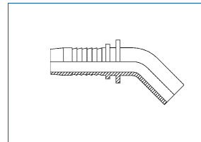
Metric Standpipe 45° Elbow
