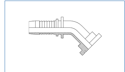
Code 62 Flange 45
