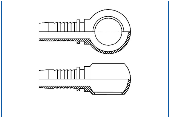
Banjo Hose End
