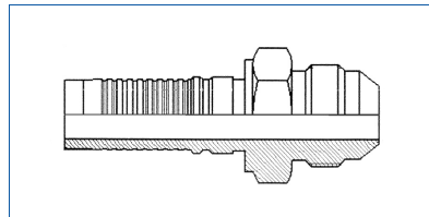
Male JIC Interlock
